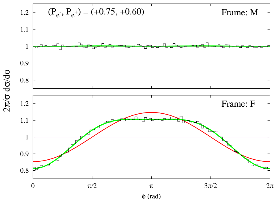
Figure 7. The azimuthal distribution same as in figure 6 for (P_{e^-}, P_{e^+}) = (+0.75, +0.60) . This is special case where frame M has flat distribution and frame F is needed for the spin determination.
