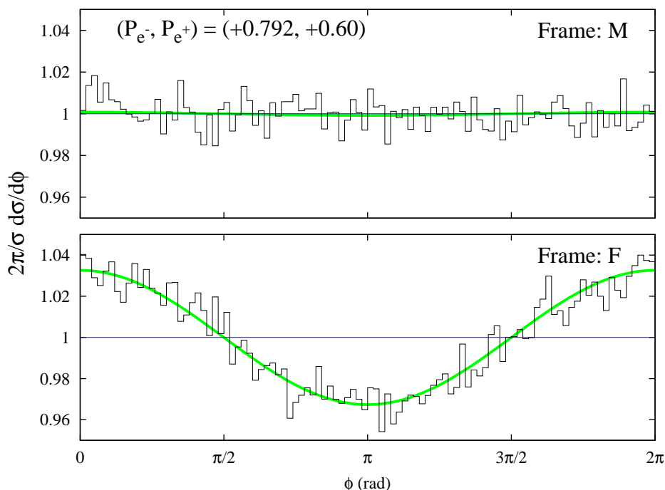
Figure 5. The azimuthal distribution same as in figure 4 for (P_{e^-}, P_{e^+}) = (+0.792, +0.60) . This is special case when the distribution is flat in frame M and frame F is needed for spin determination.
