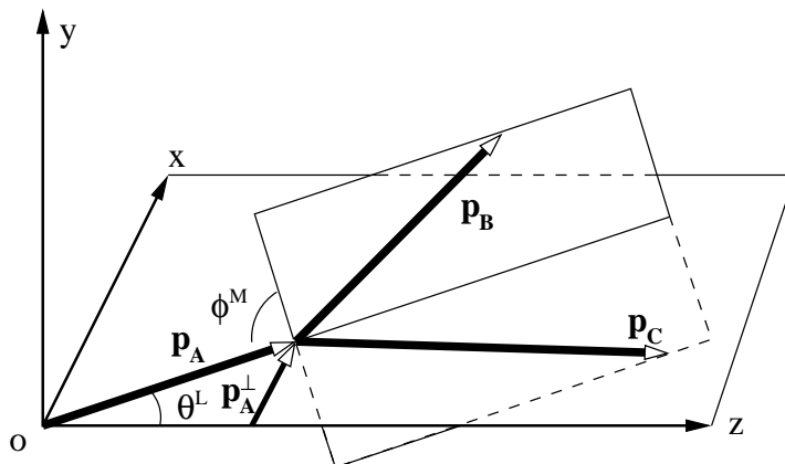
Figure 2. The momentum configuration in the laboratory frame L of the colliding beams is depicted. The angle between the production plane (the xz -plane) and the decay plane (spanned by p_B and p_C ) is the azimuthal angle \phi^M (= \phi_B^M) , which is the ordinary azimuthal angle in the frame M . This azimuthal angle has been studied in [24] and [25].
